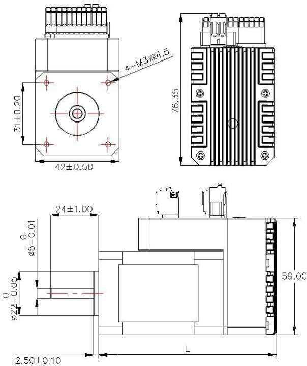
IHVS42-XX Mounting dimensions
