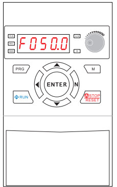
Figure 4~1 H1 series keypad
