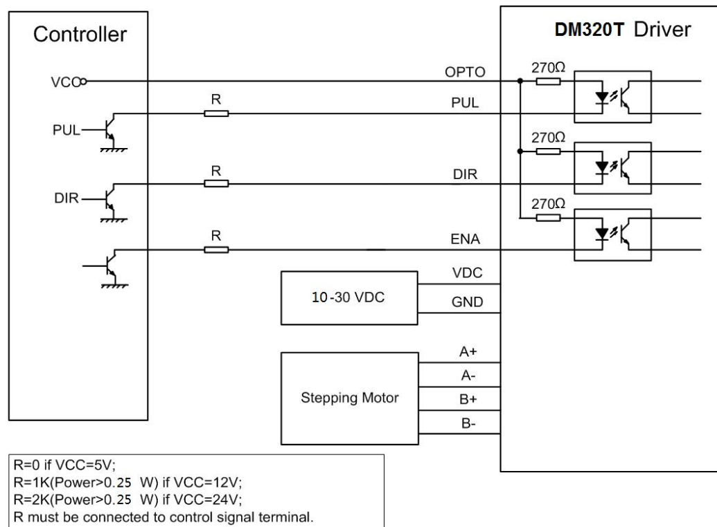
Figure 9: Typical connection
