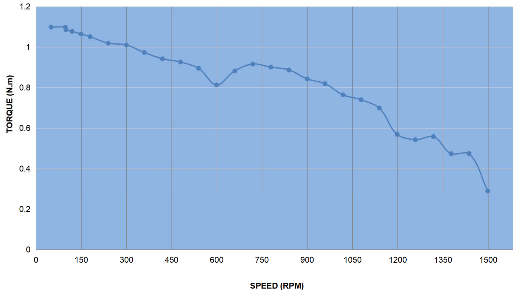
PULL OUT TORQUE CURVE OF 23E1KBK20-12
