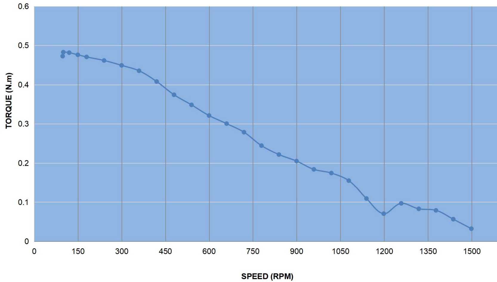
PULL OUT TORQUE CURVE OF 17E1KBK05-07
