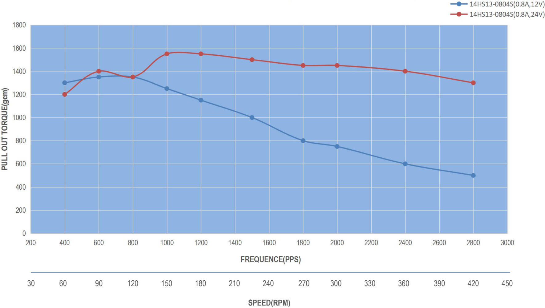
14HS13-0804S PULL OUT TORQUE(0.8A/P 12V/24V HALF STEP)
